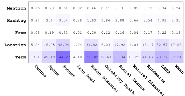
Figure 2: Matrix of mean Mutual Information values (divided by 1E + 10 for different feature types vs. topics. The last column is the average of mean values across all topics.)
