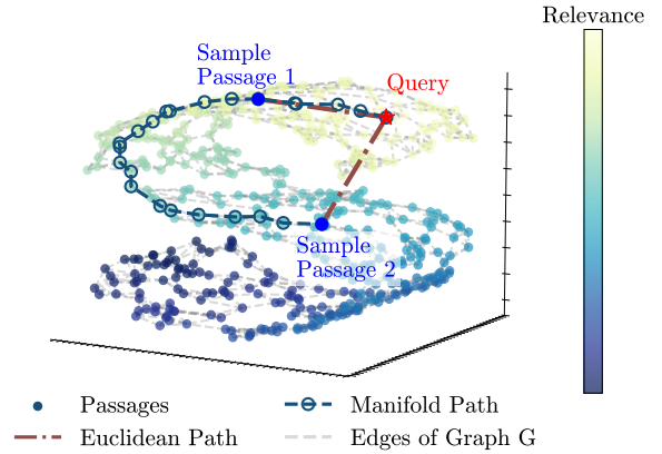
Figure 1: Example of subdimensional non-linear manifold in embedding space. Passage embeddings (dots) form a non-linear S-shaped manifold, where their relevance (indicated by color) to the query (red star) is determined by proximity along the manifold rather than Euclidean distance. Two sample passages (blue dots) have similar Euclidean distance to the query (red path) but differ in relevance. In contrast, the distance (blue path) along the weighted undirected graph G , where nodes represent passages and edges (gray dashed lines) connect each passage to its K -nearest neighbors, often better reflects the true relevance in such settings.
