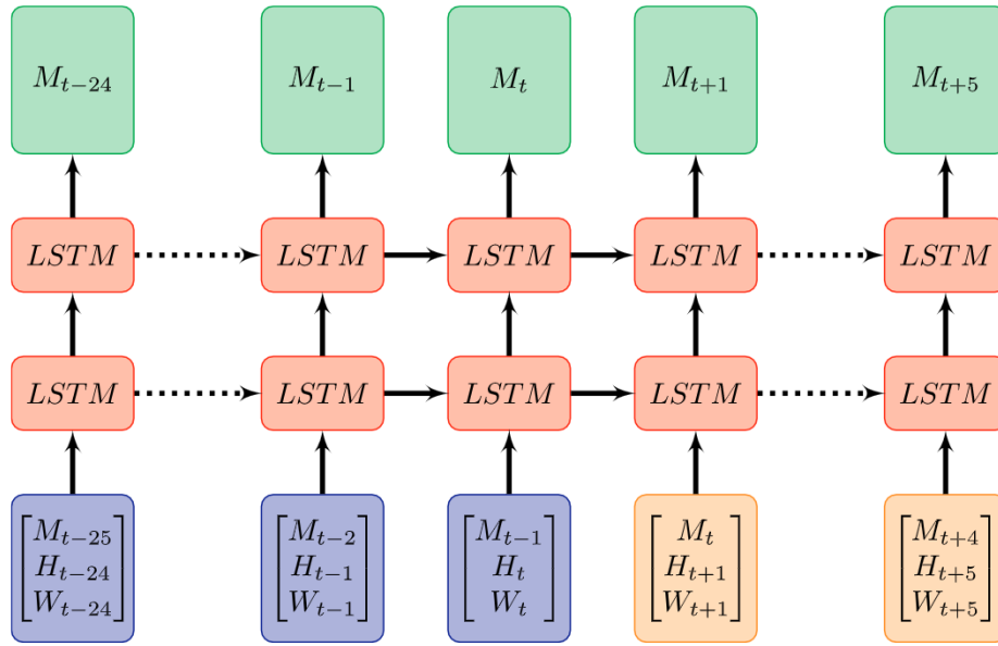
Fig. 6. Schematic of the implemented RNN. The input feature vectors (M_{t-1}, H_t, W_t) are passed into two layers of LSTM cells and results in a predicted motion state (M_t) . In the orange input vectors, the input feature M_{t-1} had an additional unobserved state value introduced to allow later inference. (For interpretation of the references to colour in this figure legend, the reader is referred to the Web version of this article.)
