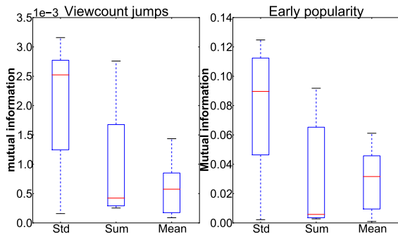
Figure 2: Box plots of mutual information grouped by feature aggregates. The most informative features are generated by std aggregation for both JUMP and EARLY .
