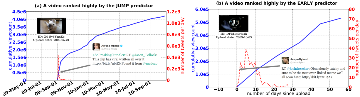
Figure 1: Examples of top predictions for JUMP and EARLY. (a) A video having less than 9000 views in its first 3 months, and then gaining 1.2 million views within 15 days (date format of x-axis: yy-mmm-dd). The insert shows a tweet linking to this video by celebrity user Alyssa Milano 2 . (b) A video with a few dozen Twitter mentions and nearly 2 \times 10^5 views in its first 15 days. Note that the video popularity continues to rise even after the tweet volume has tapered off, illustrating the prediction power of “early tweets”.
