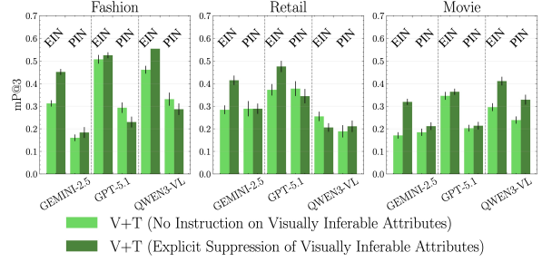
Figure 10: VLMs with item visual information (V+T) under instructions to explicit suppress visually inferable attributes (or not) showing limited latent awareness.
