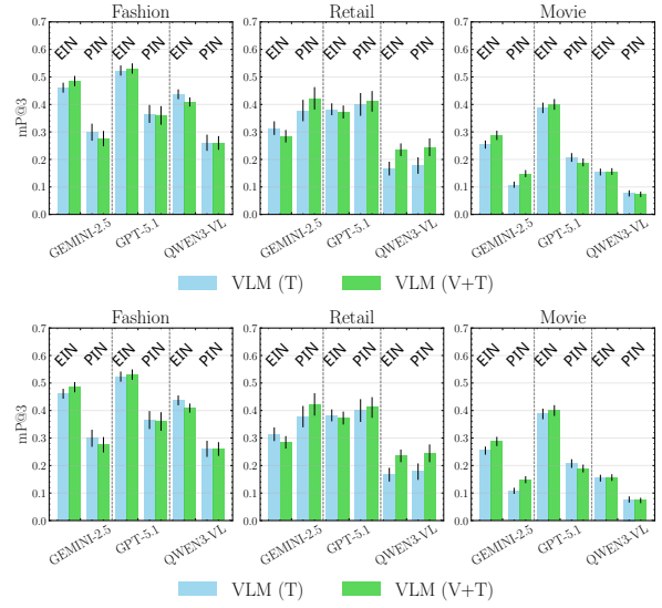
Figure 14: (Upper) Pointwise VLM performance (T) versus (V+T); (Lower) Pointwise zero-shot VLM with few-shot instruction discouraging visually inferable attributes (INSTRUCT) under V+Ts.
