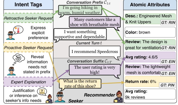
Figure 4: Ground Truth for Label Selection. Ground truth for the three proposed criteria is constructed by assigning intent tags (left) to each utterance in the full conversation (center), and selecting atomic attributes that satisfy at least one utterance (right) as ground truth.
